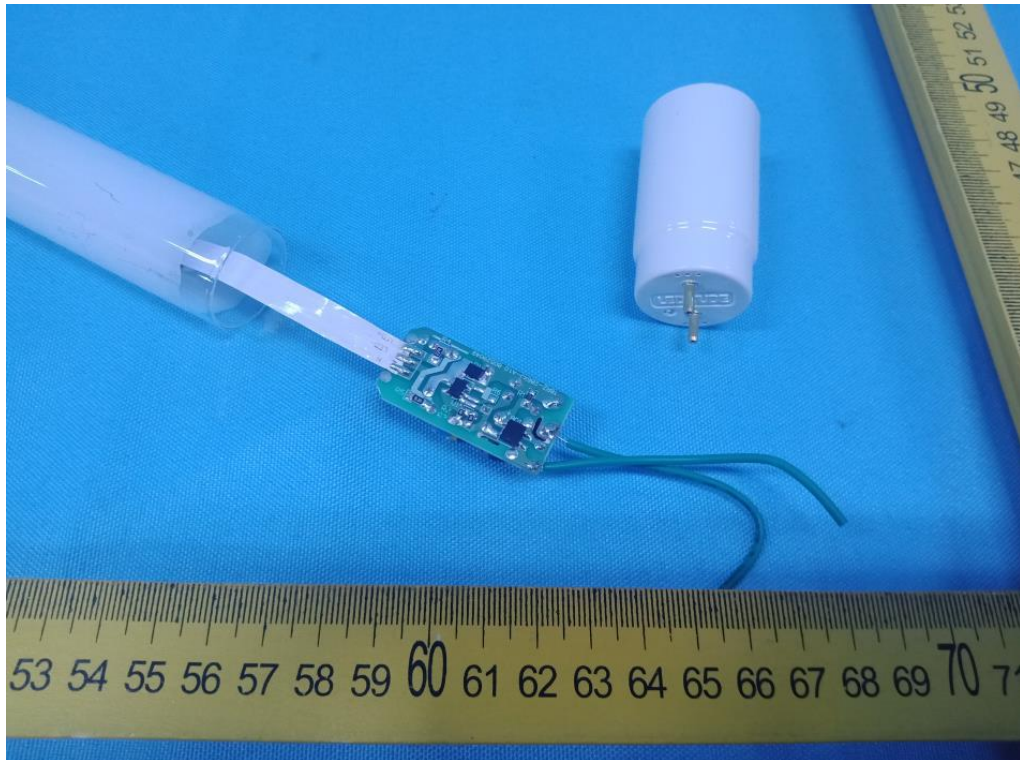
Photo 7: PCB view
