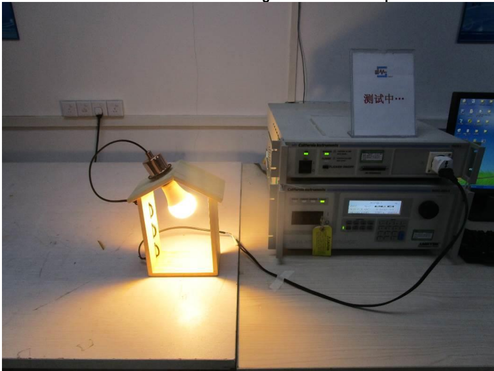
Current Harmonics /Voltage Flicker Test Setup
